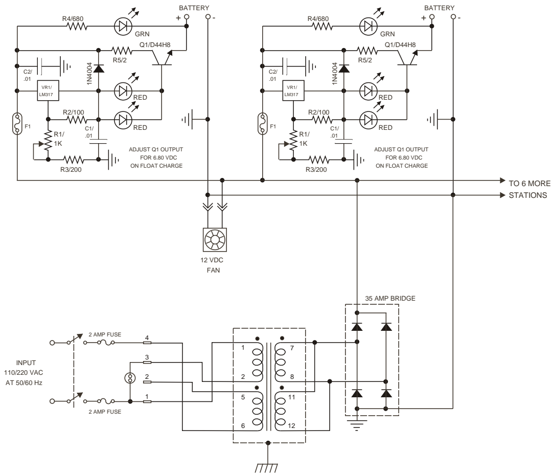
8-STATION / 6 VDC AT 1 AMP SCHEMATIC
